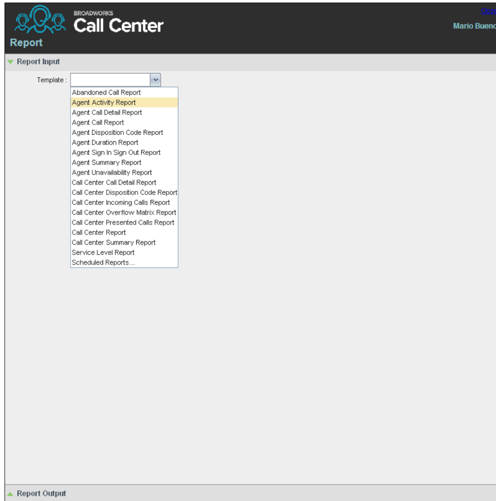
Figure 108 Report Window – Report List
