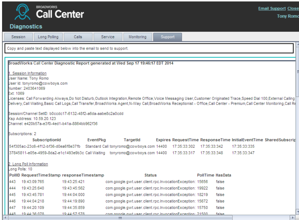
Figure 138 Diagnostic Tool – Support Tab
